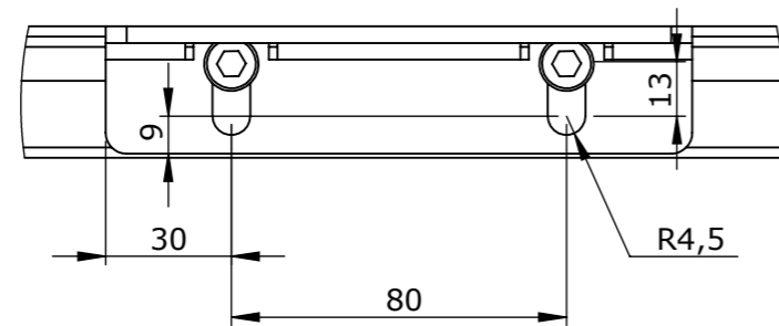
DETAIL B SCALE 1 : 2
