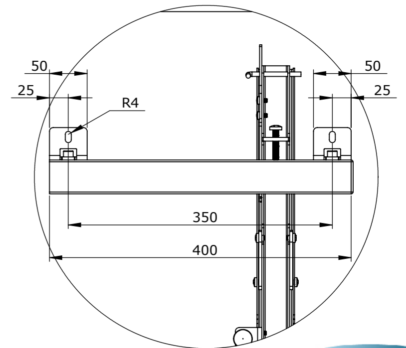
DETAIL K SCALE 1 : 5
